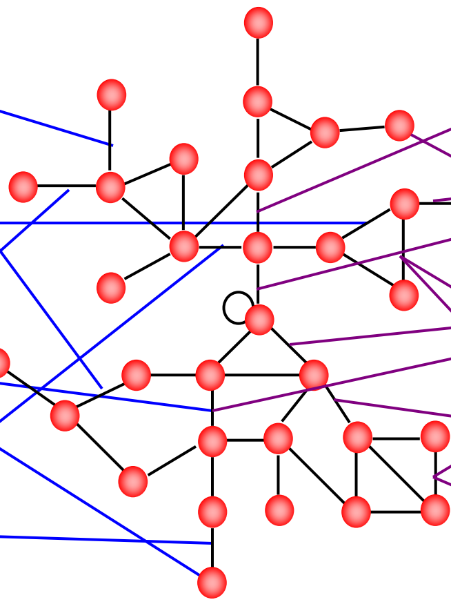
Interactome networks
